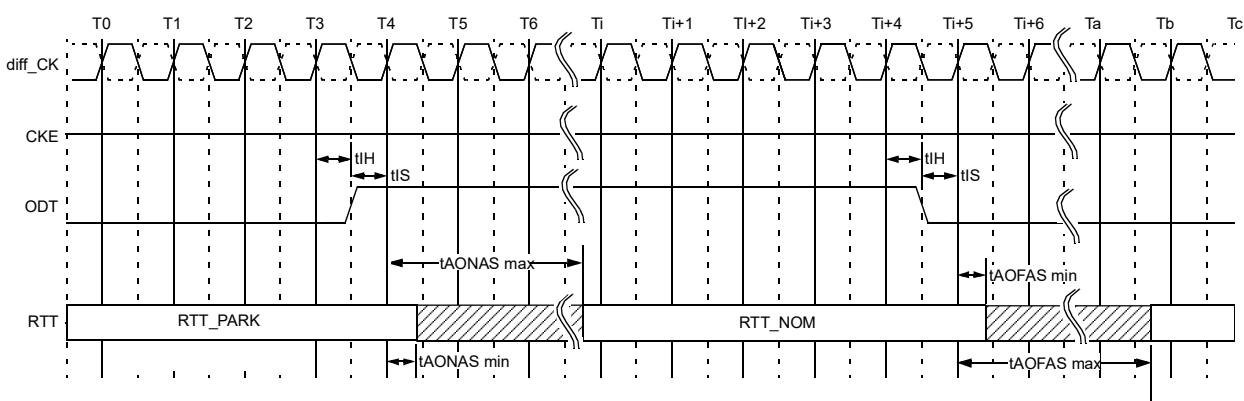
Figure 196 — Asynchronous ODT Timing on DDR4 SDRAM with DLL-off
