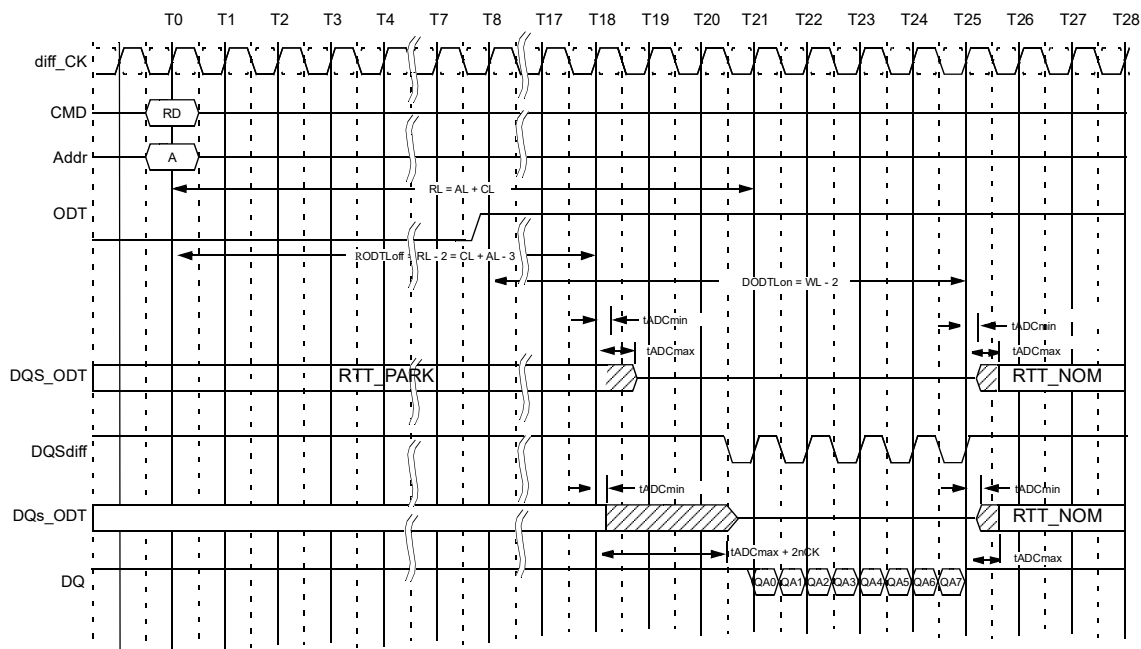
Figure 193 — Example: CL=11, PL=0; AL=CL-1=10; RL=AL+PL+CL=21; CWL=9; DODTLon=AL+CWL-2=17; DODTLoft=AL+CWL-2=17;2tCK preamble)
