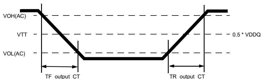
Figure 222 — Output Slew Rate Definition of Connectivity Test Mode
