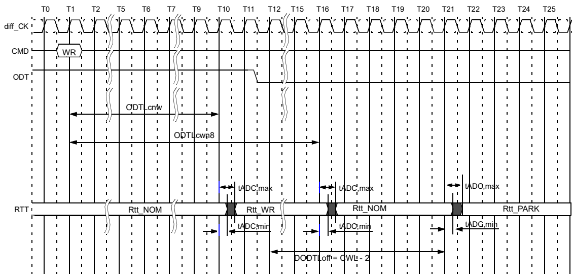
Figure 195 — Dynamic ODT overlapped with Rtt_NOM (CL=14, CWL=11, BL=8, AL=0, CRC Disabled)
