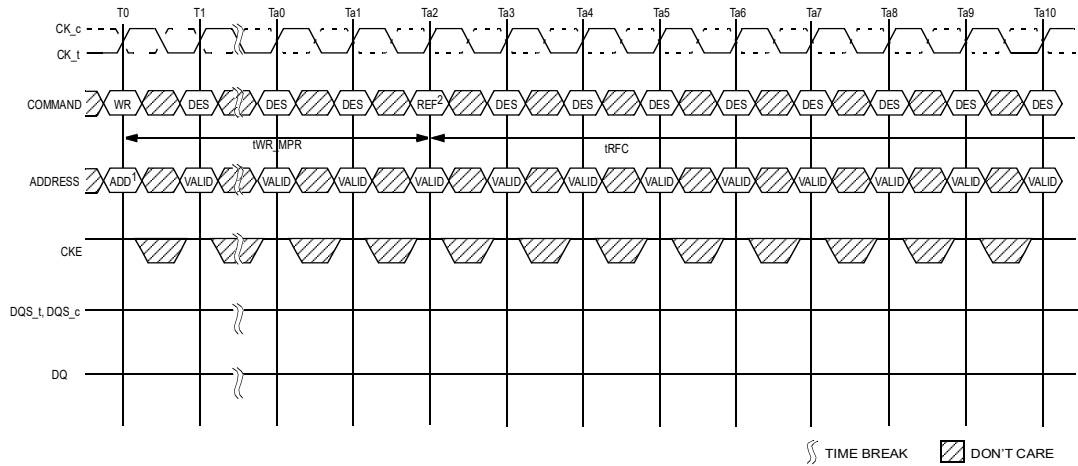
Figure 26 — Write to Refresh Command Timing
