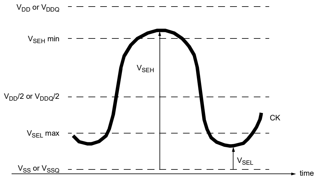
Figure 205 — Single-ended requirement for differential signals.
