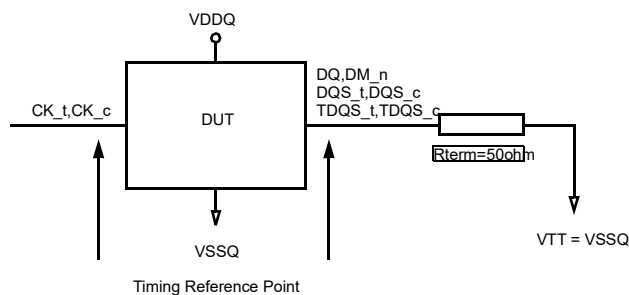
Figure 199 — ODT Timing Reference Load
