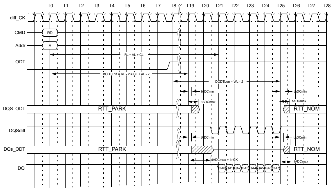
Figure 192 — Example: CL=11, PL=0; AL=CL-1=10; RL=AL+PL+CL=21; CWL=9; DODTLon=AL+CWL-2=17; DODTLoft=AL+CWL-2=17;1tCK preamble)
