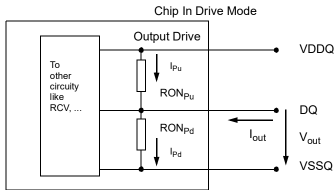
Figure 217 — Output driver
