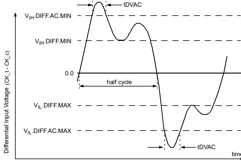
Figure 204 — Definition of differential ac-swing and “time above ac-level” t_{DVAC}
