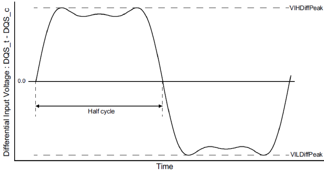
Figure 213 — Definition of differential DQS Signal AC-swing Level
