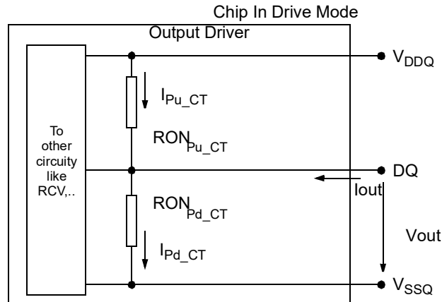
Figure 219 — Output Driver
