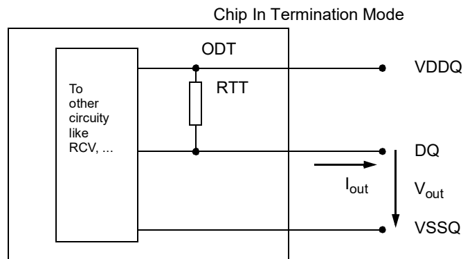
Figure 189 — On Die Termination
