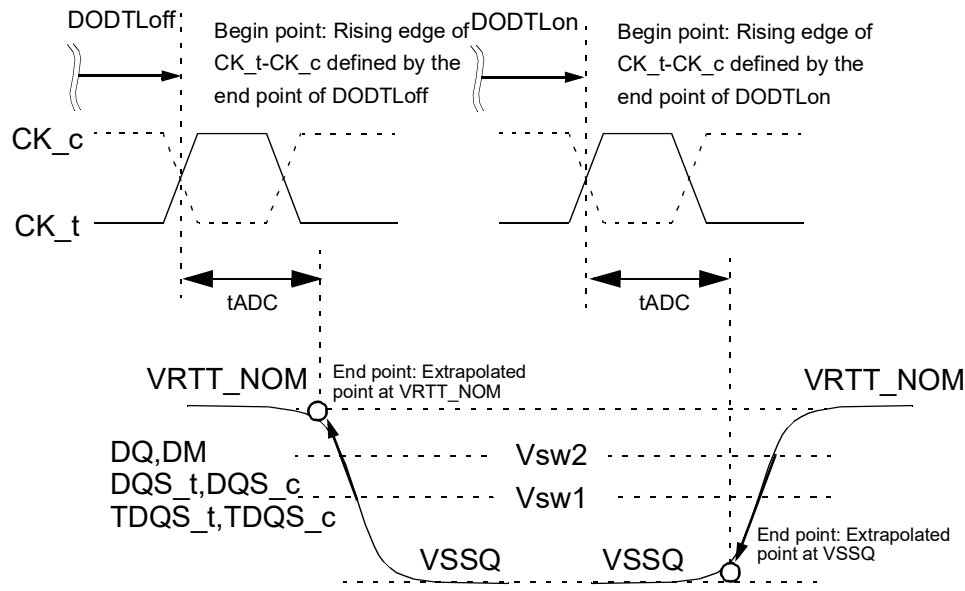
Figure 200 — Definition of t_{ADC} at Direct ODT Control
