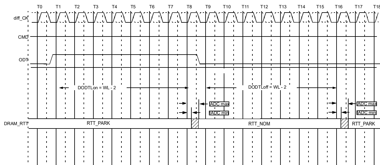
Figure 190 — Synchronous ODT Timing Example for CWL=9, AL=0, PL=0; DODTLon=WL-2=7; DODTLoFF=WL-2=7
