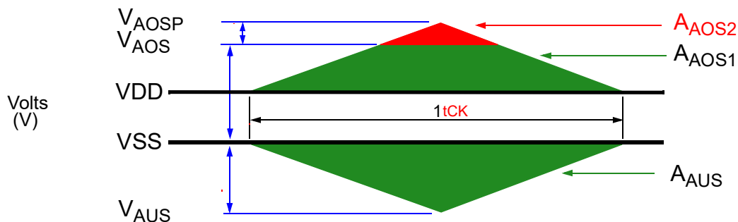
Figure 206 — Address, Command and Control Overshoot and Undershoot Definition
