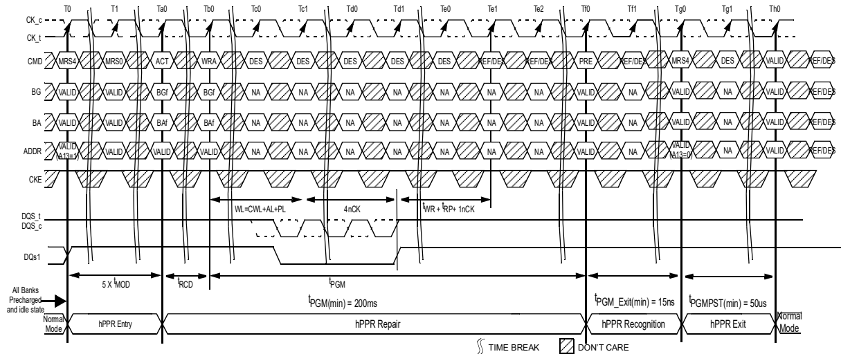
Figure 185 — Hard Fail Row Repair (WRA Case)
