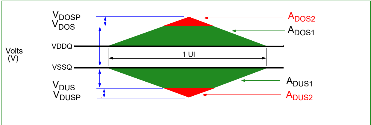
Figure 208 — Data, Strobe and Mask Overshoot and Undershoot Definition
