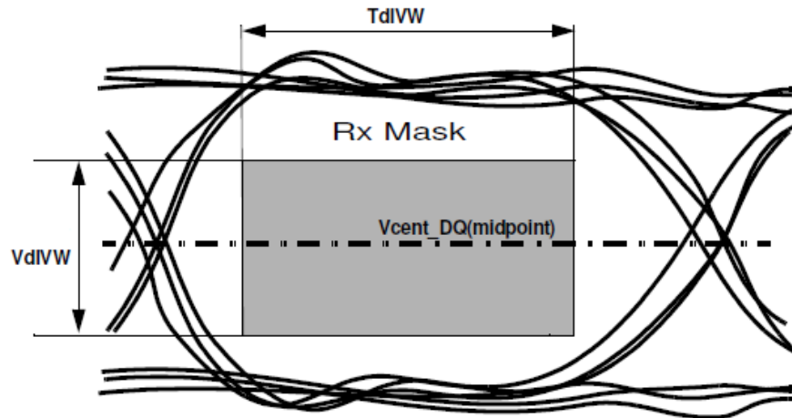
Figure 227 — DQ Receiver(Rx) compliance mask
