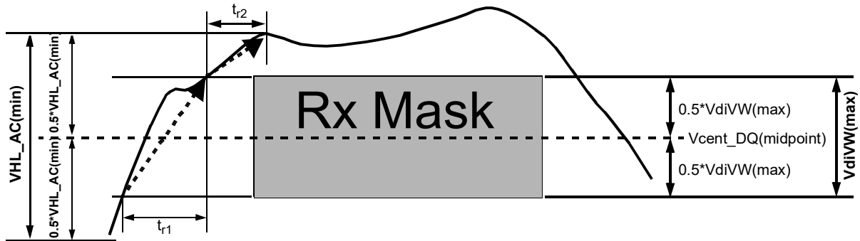
Figure 230 — Slew Rate Conditions For Rising Transition
