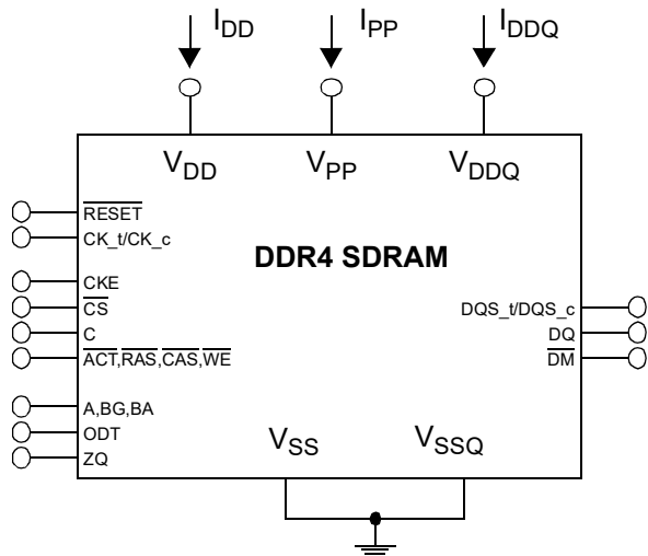
Figure 224 — Measurement Setup and Test Load for IDD, IPP and IDDQ Measurements
