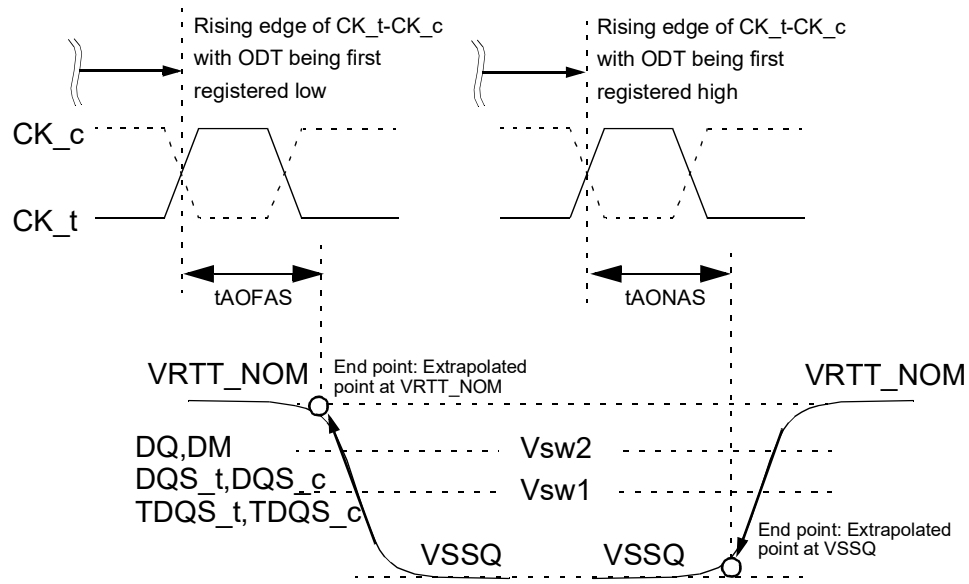
Figure 202 — Definition of t_{AOFAS} and t_{AONAS}
