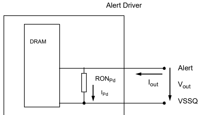
Figure 218 — Functional Representation of the Output Buffer
