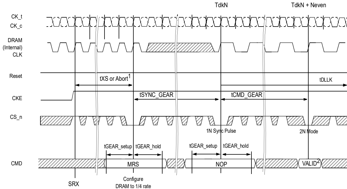
Figure 66 — Gear down (2N) mode entry sequence during initialization
