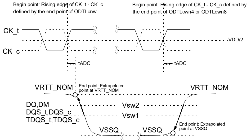
Figure 201 — Definition of t_{ADC} at Dynamic ODT Control
