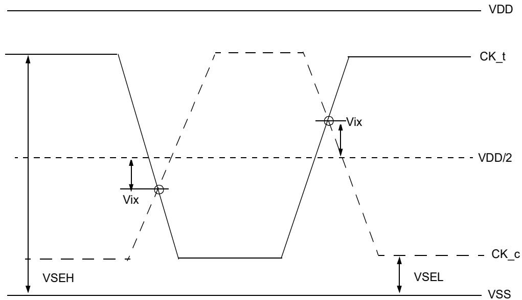
Figure 211 — Vix Definition (CK)
