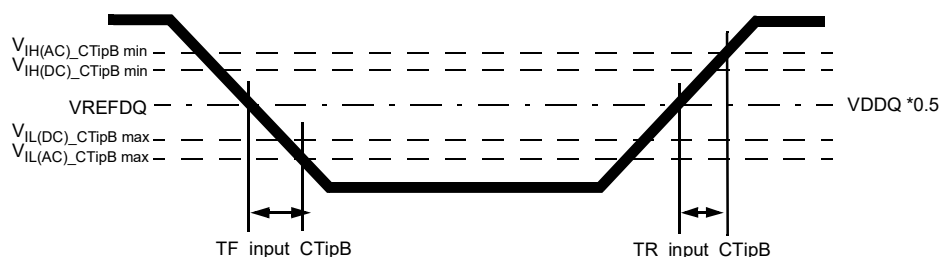
Figure 181 — Input B Slew Rate Definition
