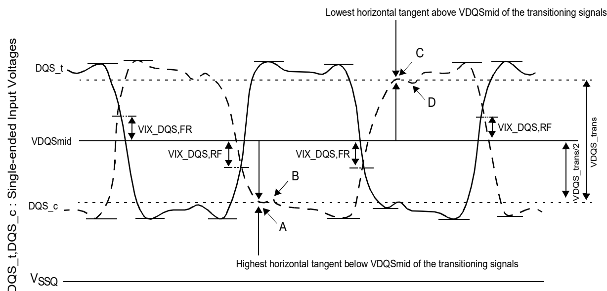
Figure 215 — Vix Definition (DQS)
