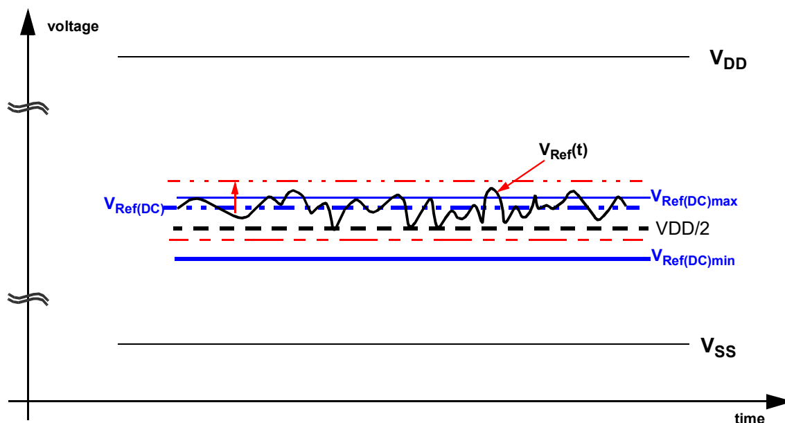
Figure 203 — Illustration of V_{REF}(DC) tolerance and V_{REF} AC-noise limits
