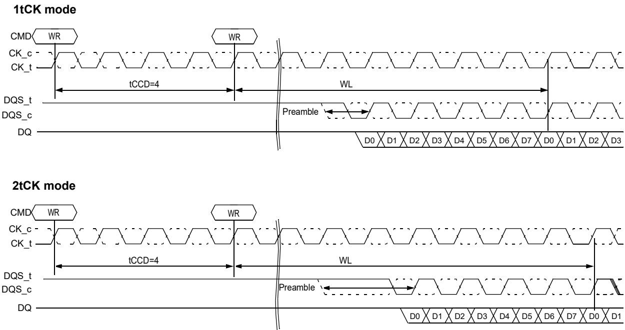
Figure 76 — tCCD=4 (AL=PL=0) of 1 tCK and 2 tCK
