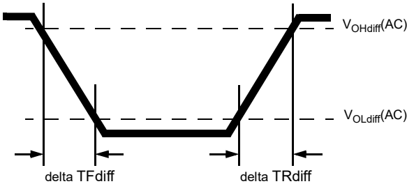
Figure 221 — Differential Output Slew Rate Definition
