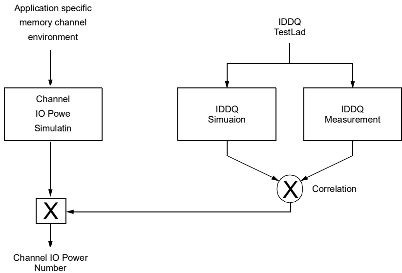
Figure 225 — Correlation from simulated Channel IO Power to actual Channel IO Power supported by IDDQ Measurement.
