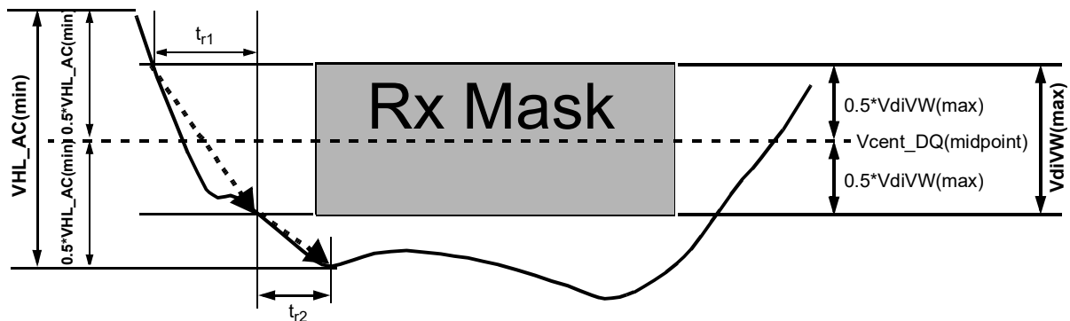
Figure 231 — Slew Rate Conditions For Falling Transition
