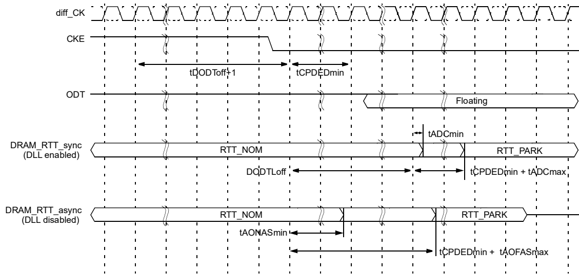
Figure 197 — ODT timing for power down entry with ODT buffer disable mode
