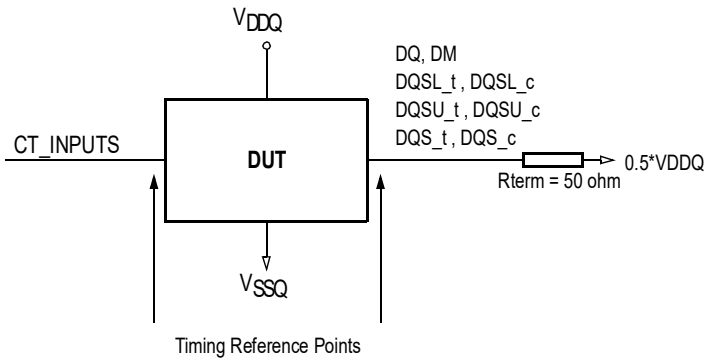
Figure 223 — Connectivity Test Mode Timing Reference Load
