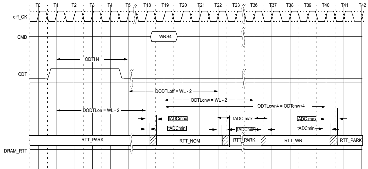
Figure 191 — Synchronous ODT example with BL=4, CWL=9, AL=10, PL=0; DODTLon/off=WL-2=17, ODTcnw=WL-2=17
