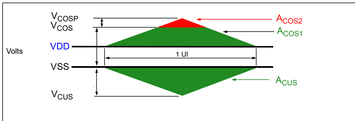
Figure 207 — Clock Overshoot and Undershoot Definition
