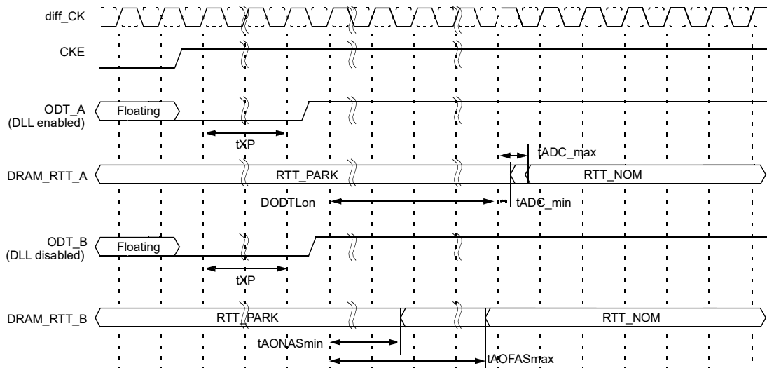
Figure 198 — ODT timing for power down exit with ODT buffer disable mode
