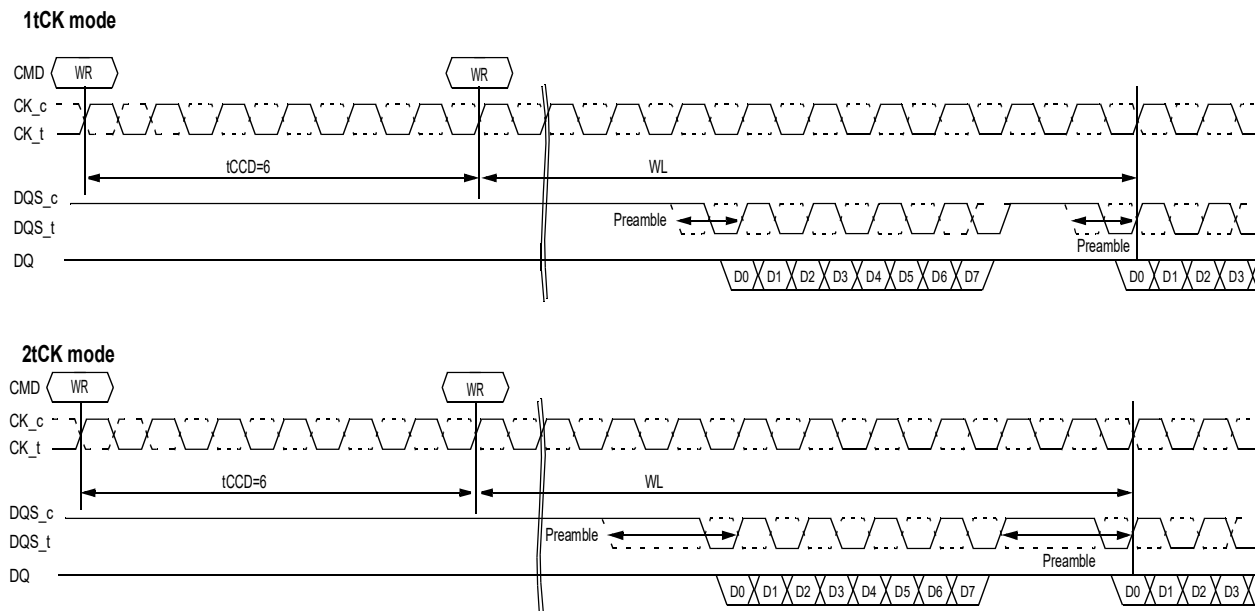
Figure 78 — tCCD=6 (AL=PL=0) of 1 tCK and 2 tCK
