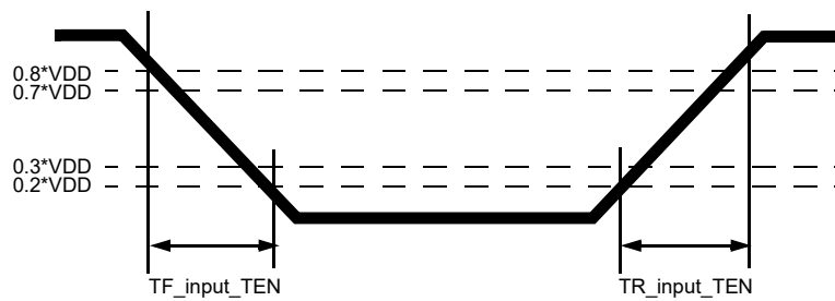
Figure 179 — TEN Input Slew Rate Definition
