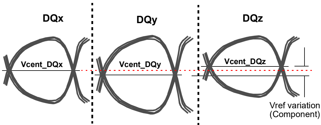
Figure 228 — Vcent_DQ Variation to Vcent_DQ(midpoint)
