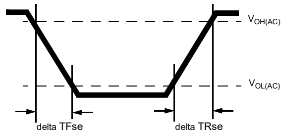
Figure 220 — Single-ended Output Slew Rate Definition
