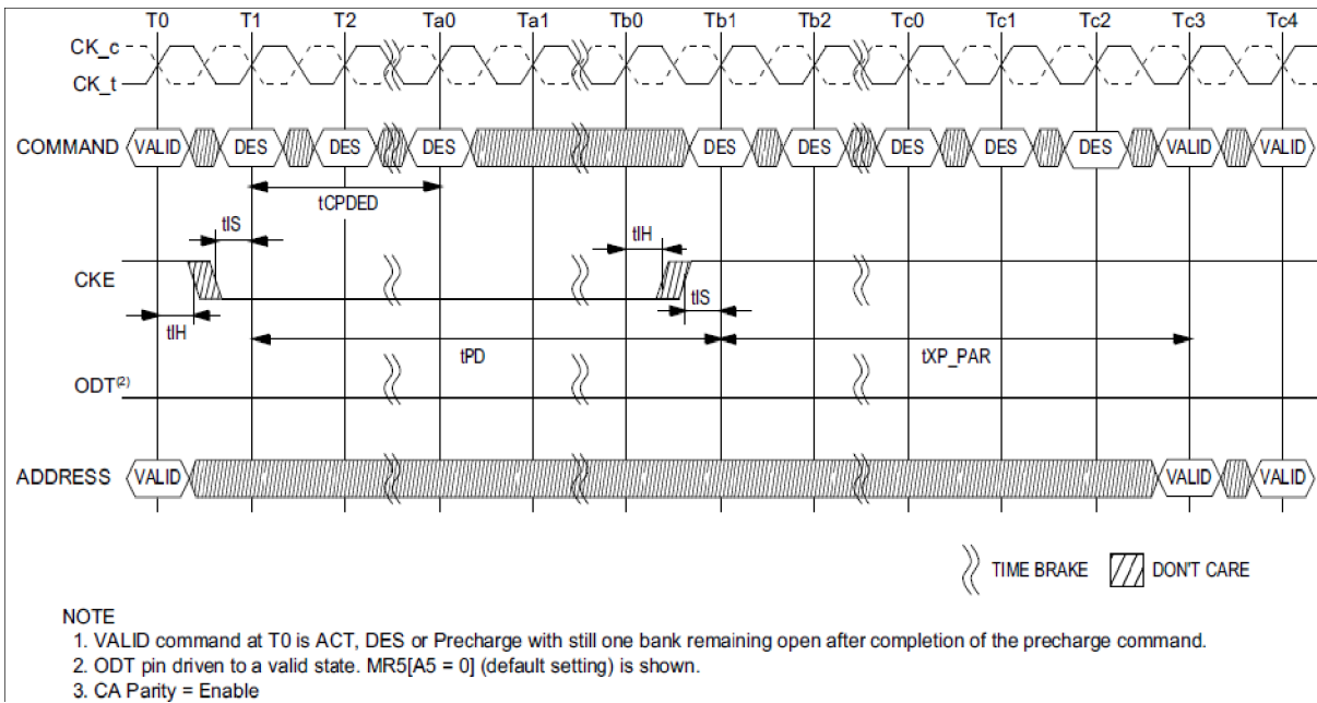
Figure 173 — Power Down Entry and Exit Timing with C/A Parity
