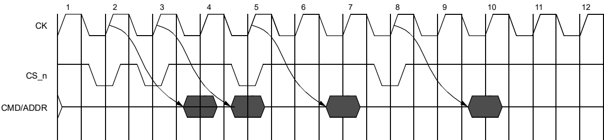
Figure 40 — CAL operational timing for consecutive command issues
