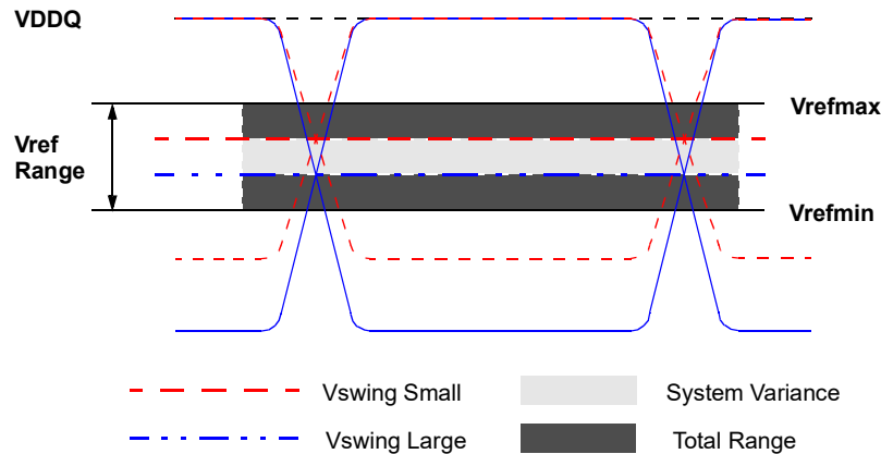
Figure 28 — Vref operating range(Vrefmin, Vrefmax)
