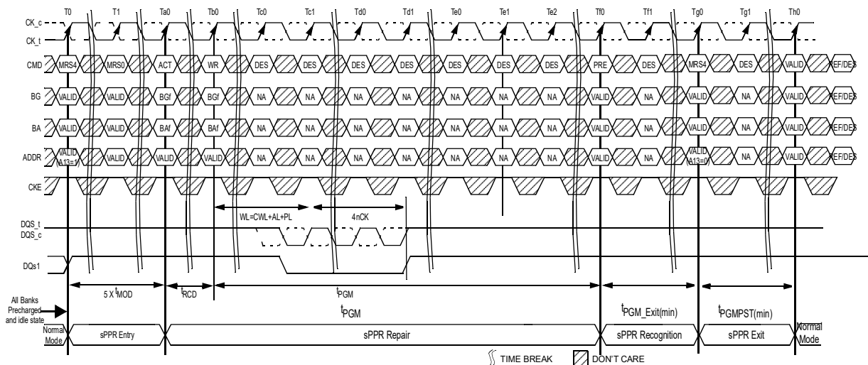
Figure 187 — Fail Row Soft PPR (WR Case)
