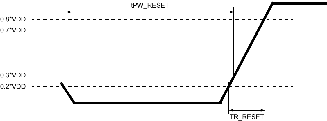
Figure 212 — RESET_n Input Slew Rate Definition
