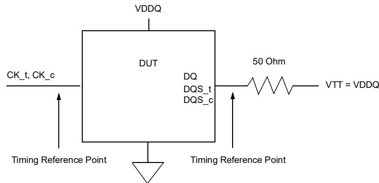
Figure 226 — Reference Load for AC Timing and Output Slew Rate
